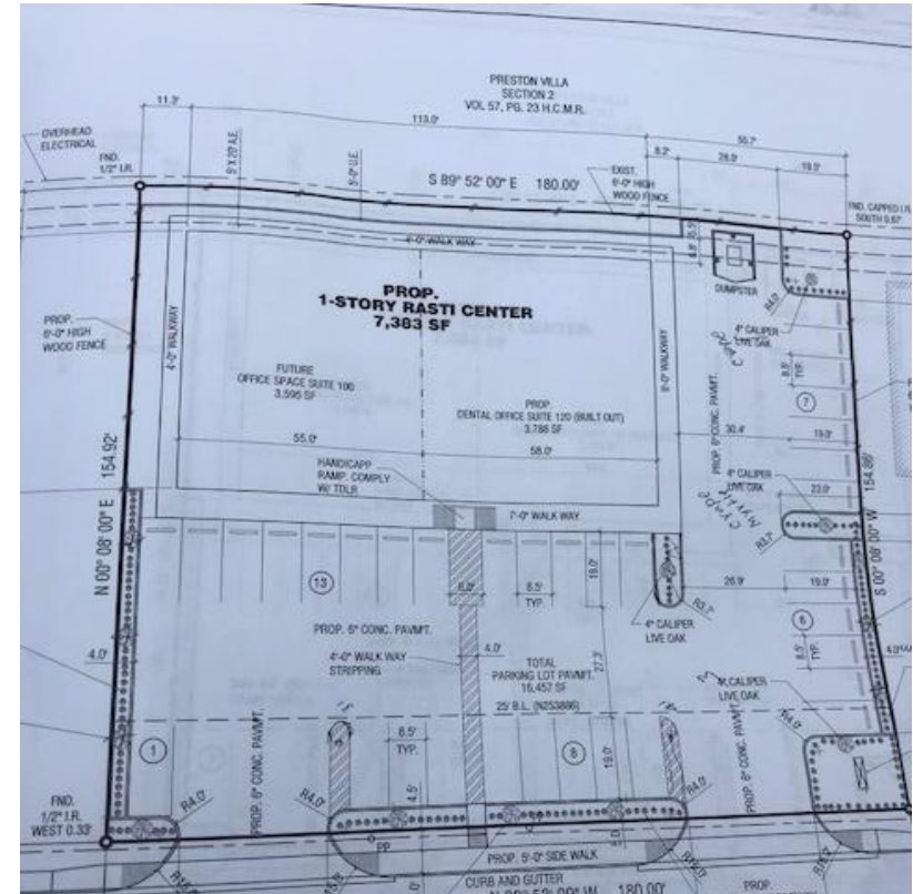
SITE PLAN FOR 2525 SOUTHMORE
